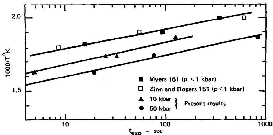
Fig 3 Time to Explosion for HMX (Ref 9a)
